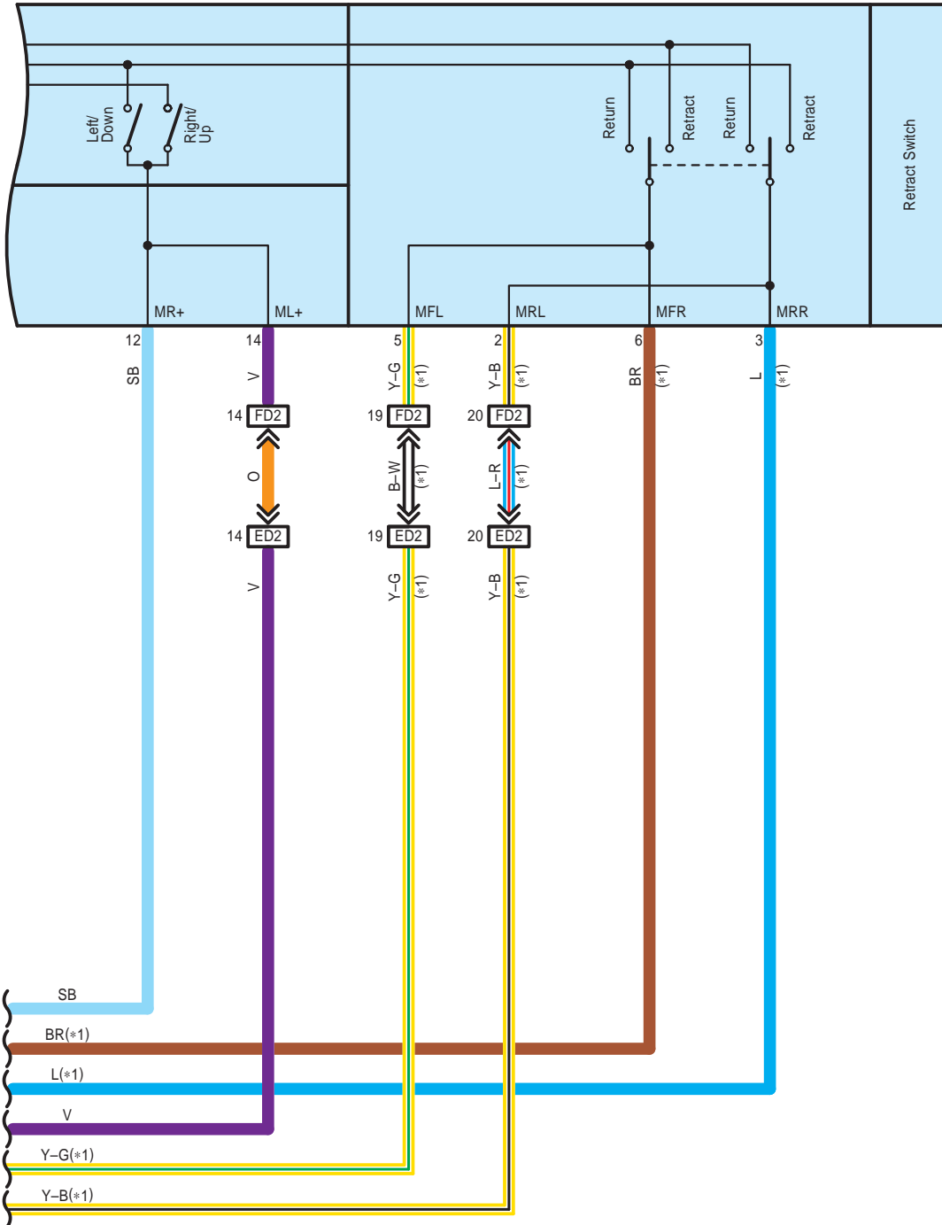
F7 Outer Mirror Switch Assembly
