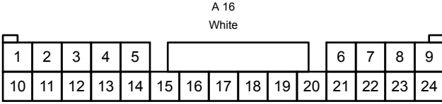
(Front Turn Signal Light, Clearance Light, Daytime Running Light and Front Fog Light)
